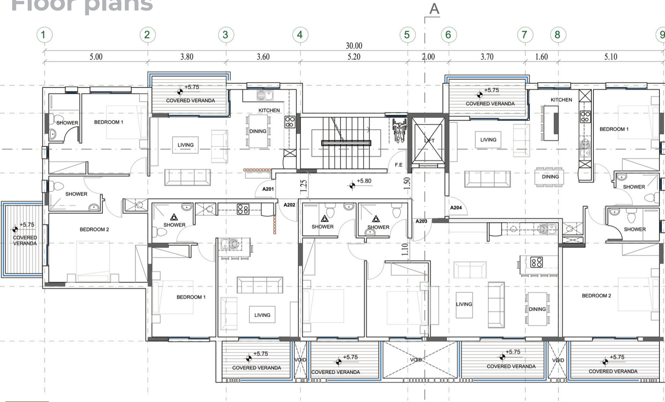
Block A - Second Floor A
