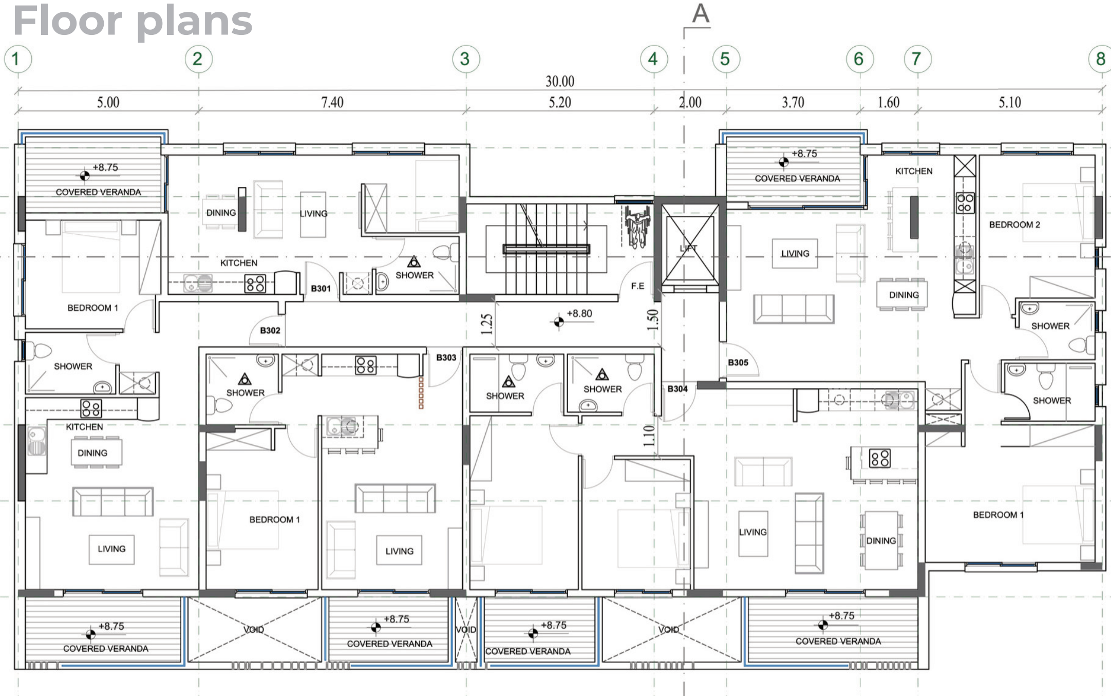
Block B - Third Floor
