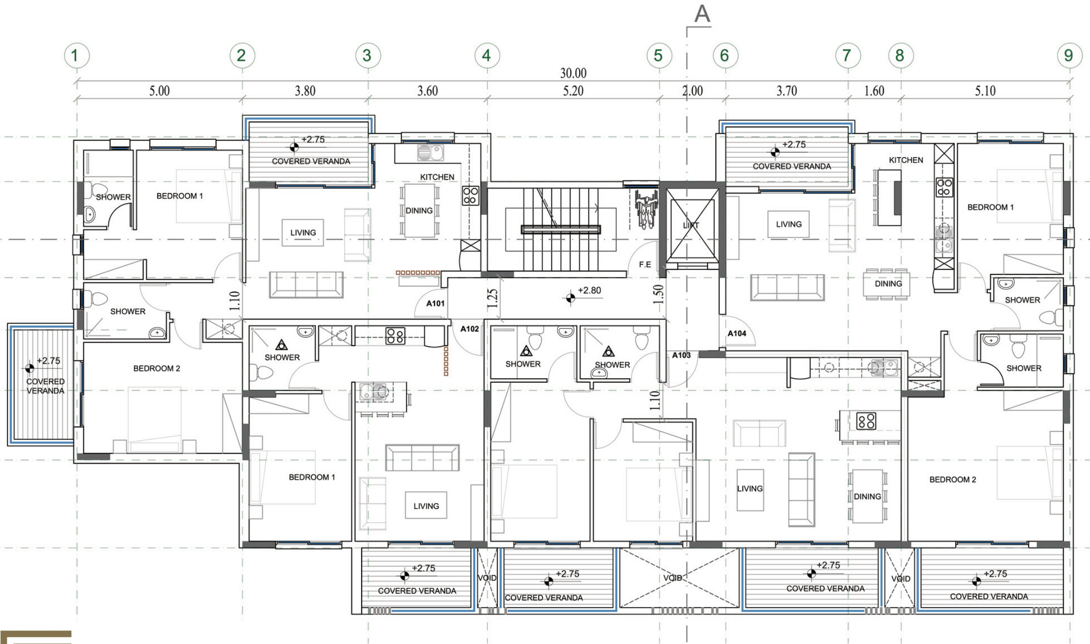
Block A - First Floor
