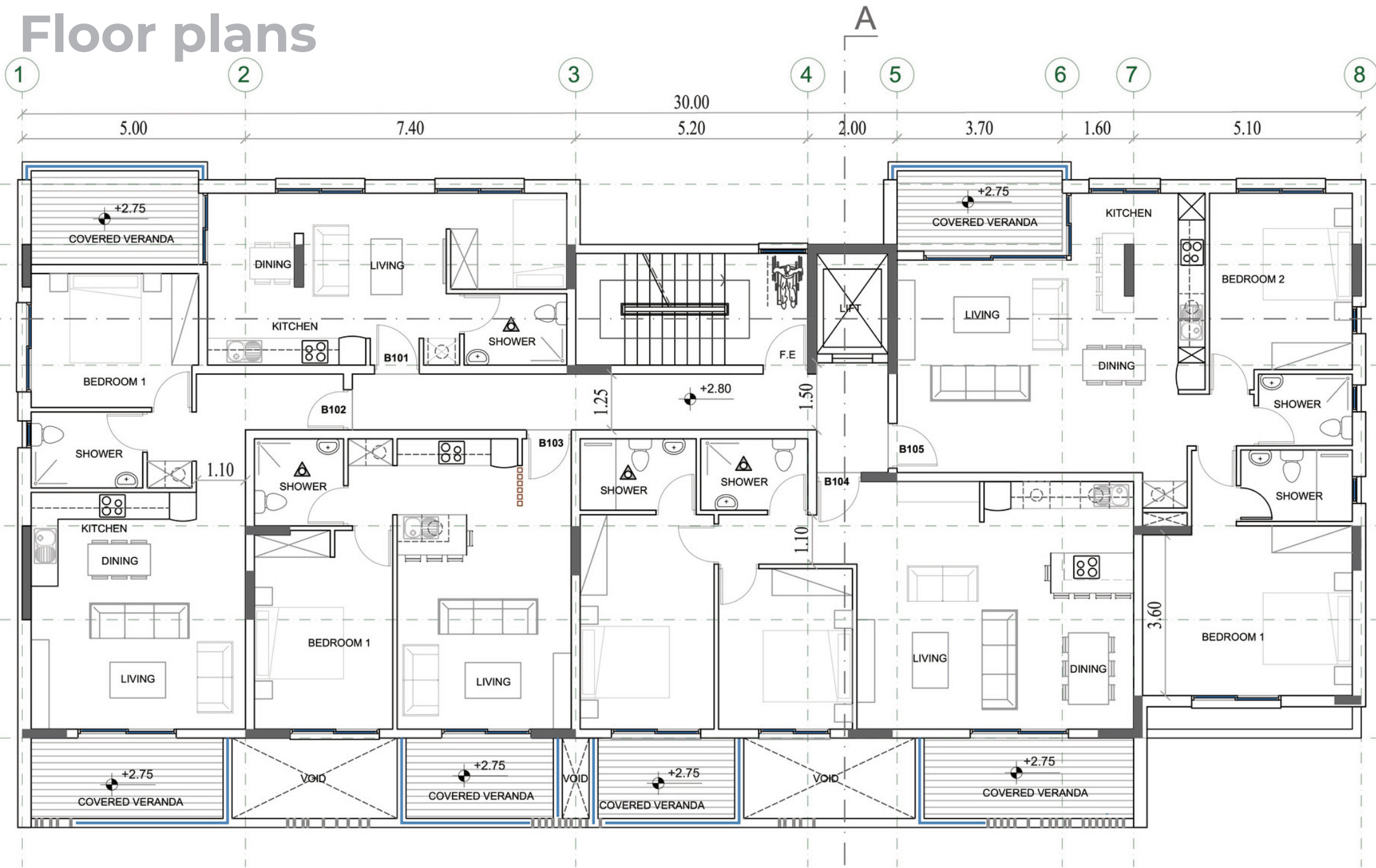
Block B - First Floor A
