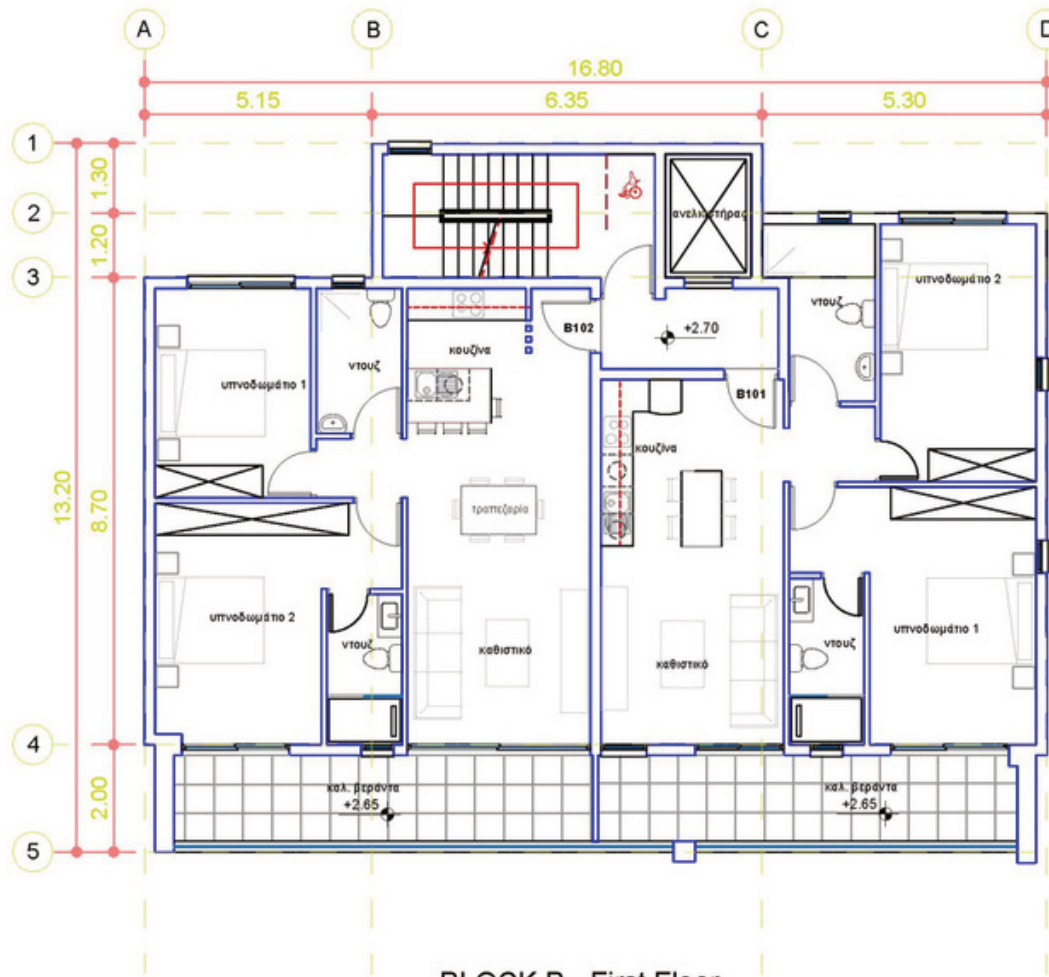
BLOCK B - First Floor
