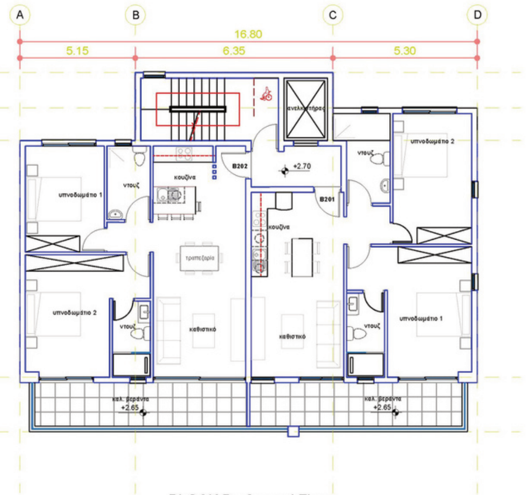
BLOCK B - Second Floor
