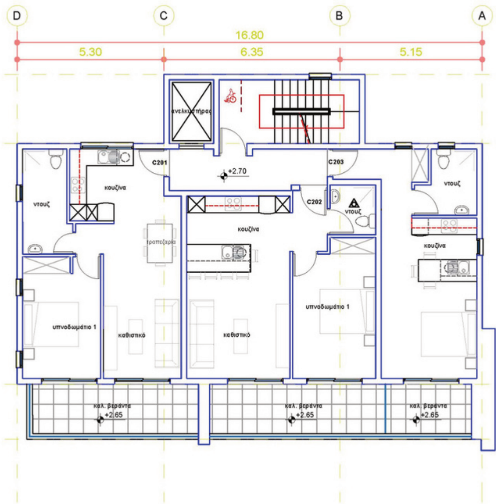
BLOCK C - Second Floor
